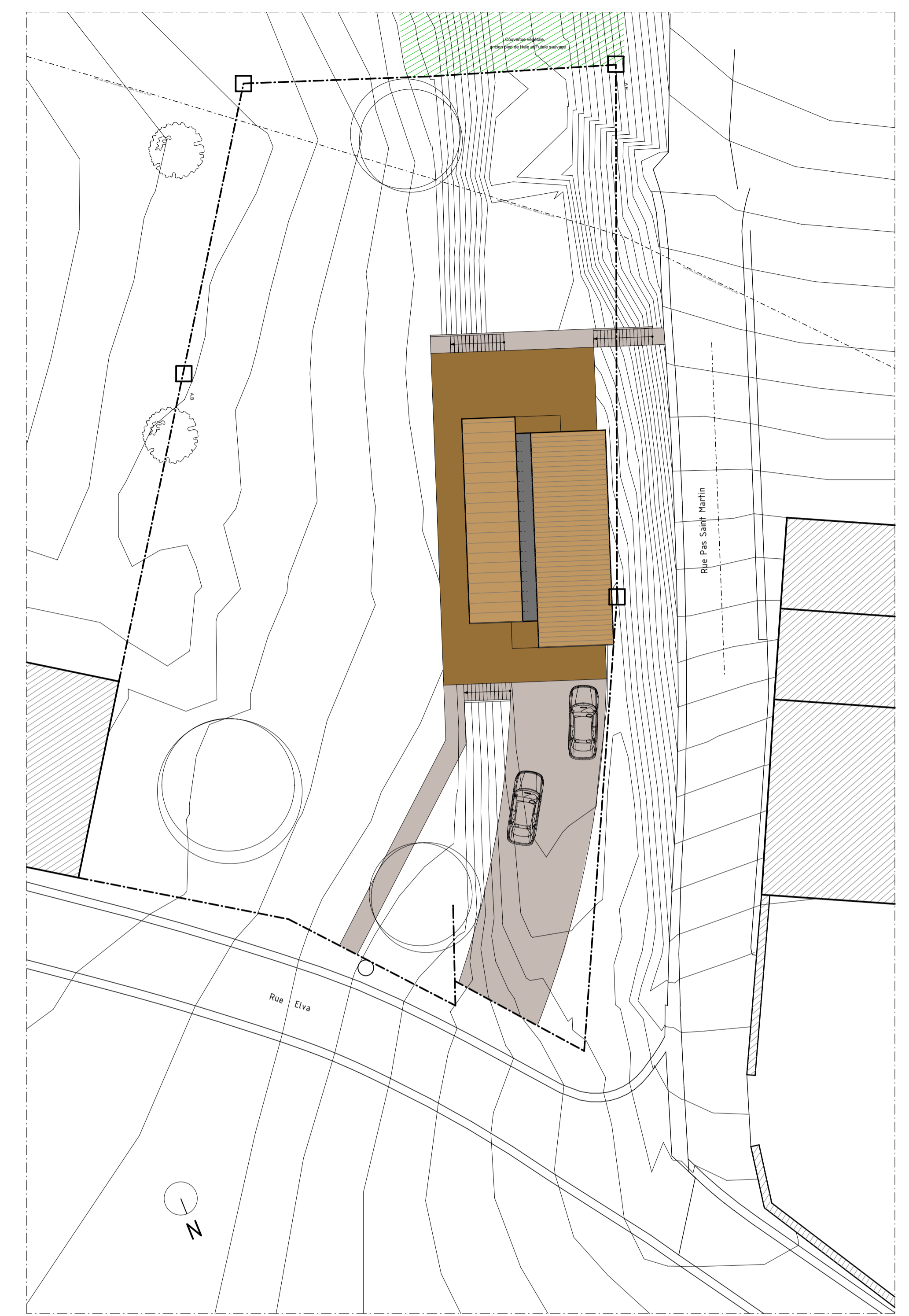
IMPLANTATION 0 200 500 1000 cm
